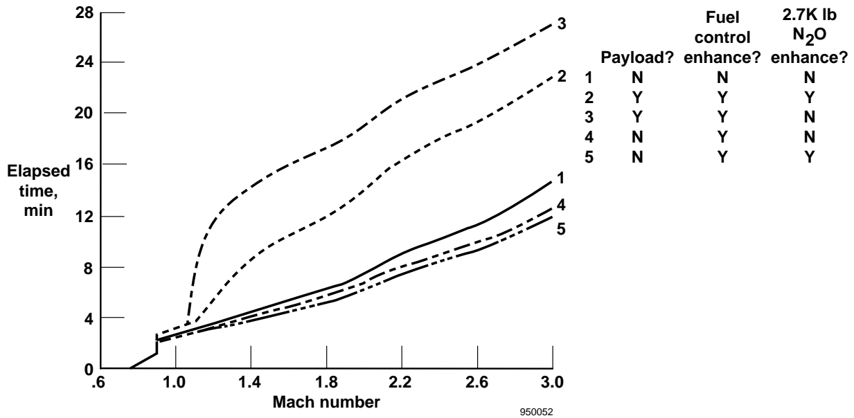
FIGURE 14. ELAPSED TIME TO ACCELERATE TO MACH 3 AND AN ALTITUDE OF 70,000 FT (21,336 M) USING VARIOUS PAYLOAD AND ENHANCEMENT OPTIONS; 500 KEAS CLIMB SCHEDULE USED.
