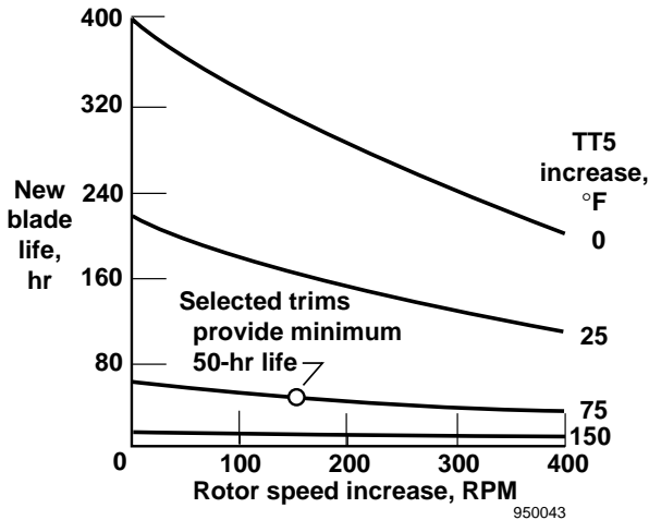
FIGURE 6. SECOND STAGE TURBINE BLADE LIFE LOSS AS A FUNCTION OF INCREASING ROTOR SPEED AND TURBINE EXHAUST TEMPERATURE.
