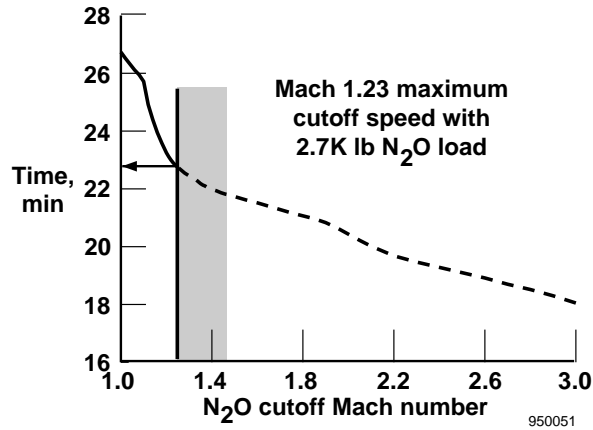
FIGURE 13. TIME TO REACH MACH 3 AND AN ALTITUDE OF 70,000 FT (21,336 M) FROM MACH 0.75 AND AN ALTITUDE OF 25,000 FT (7620 M) AS A FUNCTION OF N 2 O CUTOFF MACH NUMBER; 500 KEAS CLIMB SCHEDULE AND PAYLOAD USED.
