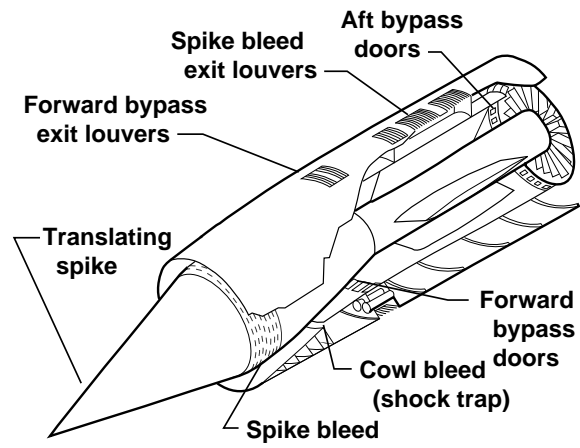
FIGURE 4. INLET CUTAWAY VIEW WITH FEATURES.
