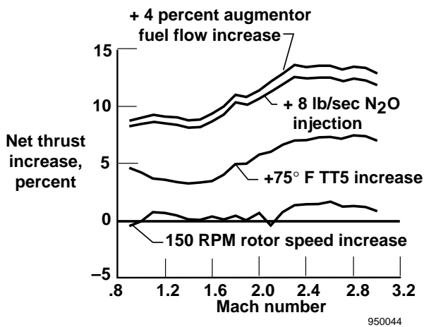
FIGURE 7. CUMULATIVE NET THRUST INCREASES FROM INDIVIDUAL THRUST ENHANCEMENT OPTIONS FOR 500 KEAS.
