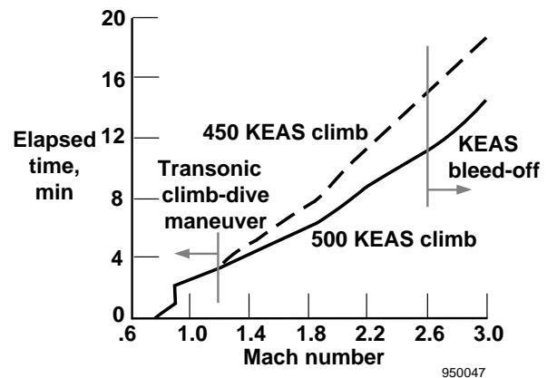
FIGURE 10. ELAPSED TIME TO ACCELERATE TO MACH 3 AND AN ALTITUDE OF 70,000 FT (21,336 M) USING TWO DIFFERENT CLIMB SCHEDULES; NO ENHANCEMENT AND NO PAYLOAD USED.
