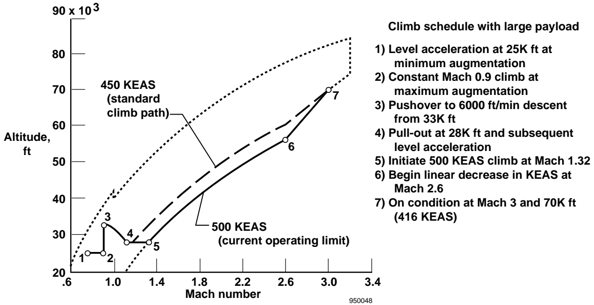
FIGURE 11. THE SR-71 FLIGHT ENVELOPE WITH RECOMMENDED 500 KEAS CLIMB SCHEDULE PROCEDURE.
